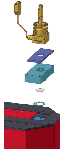
Mounting of the LLK-D fiber connector on the EC-PM
